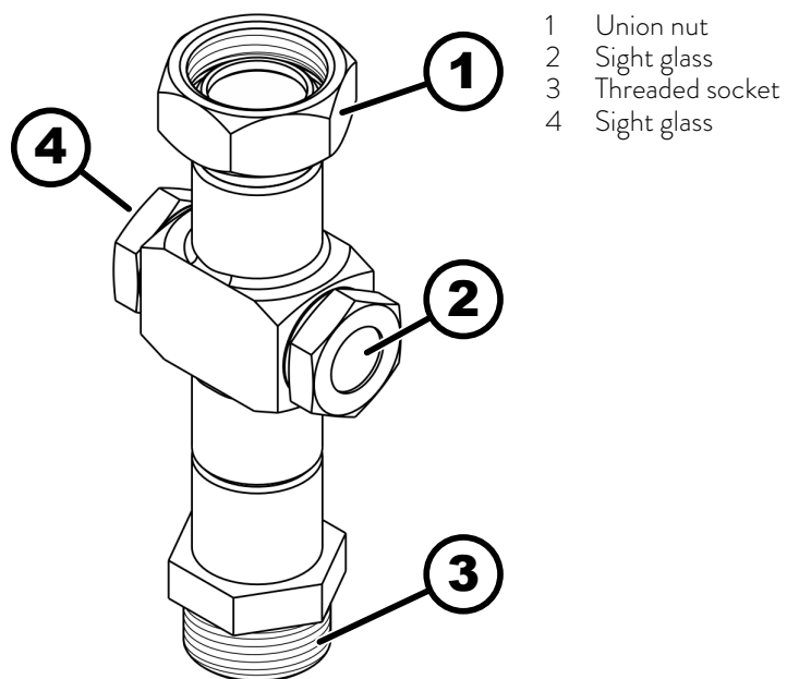
Fig. 1: Sight Glass
